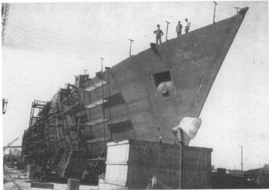
JARVIS UNDER CONSTRUCTION, 1970 AVONDALE SHIPYARDS, NEW ORLEANS
